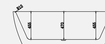
Capri Large 1700 x 800mm Bath
