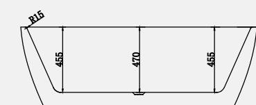
Capri Small 1500 x 800mm Bath
